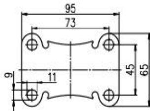
Plate Fixed
