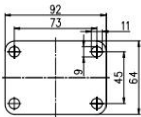
Plate Swivel
