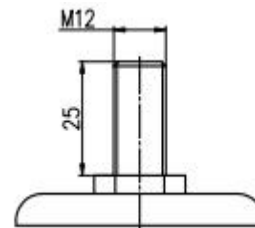
Threaded Stem
