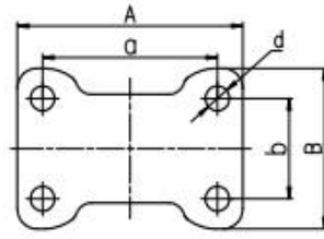
Plate Fixed
